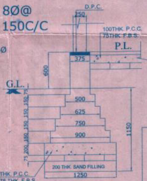
DET. OF BRICK FOUNDATION (250)
